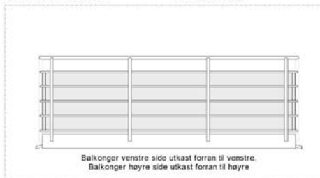
DETALJOPPRISS FRONT 1:20
